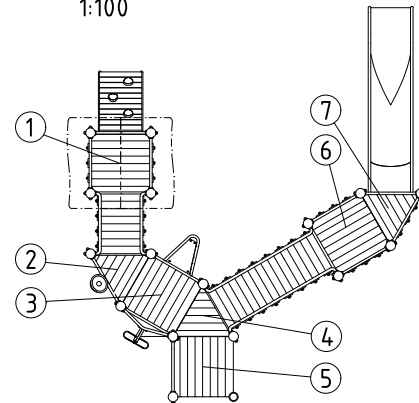
platform orientation/numbers 1:100
