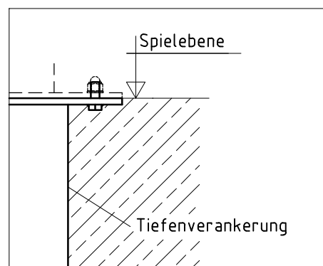
Detail Fundamentanker 1:10
