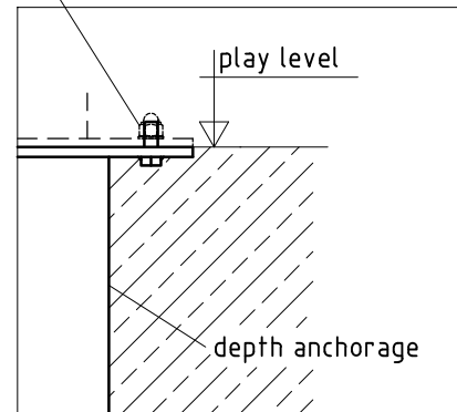
detail depth anchoring 1:10
