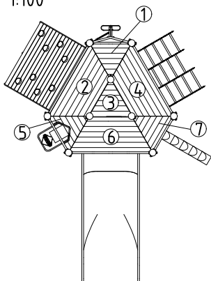
platform orientation/numbers 1:100
